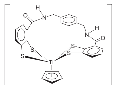
Fig. 1 Molecular structure of the anion in [\text{NMe}_4][\text{TiCp}(\text{L}^1)] .
